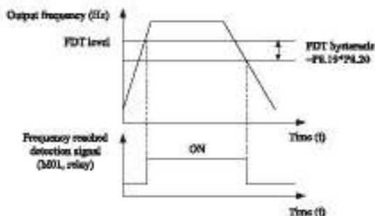
Figure 4-14 FDT level
