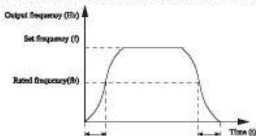
Figure 4-1 S-curve acceleration/deceleration B
