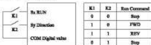
Figure 4-8 Setting of two-line mode 1
