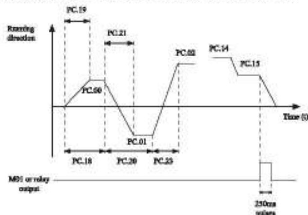
Figure 4-28 Simple PLC when used as frequency source
